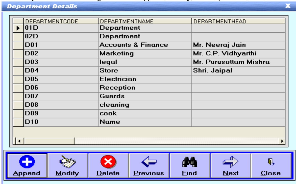
Figure 11: Department Master-1
