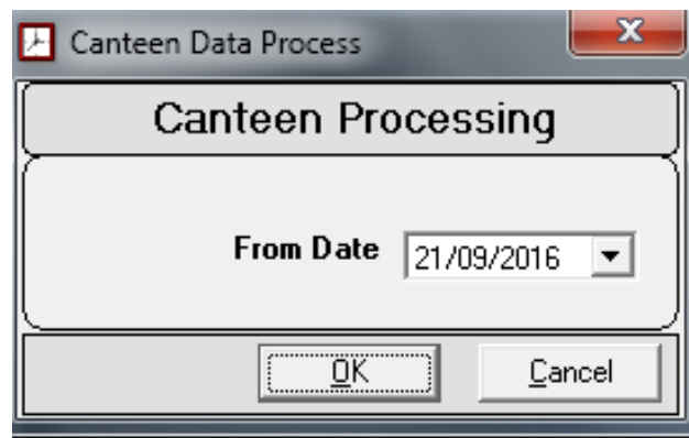
Figure 45: Canteen Processing
