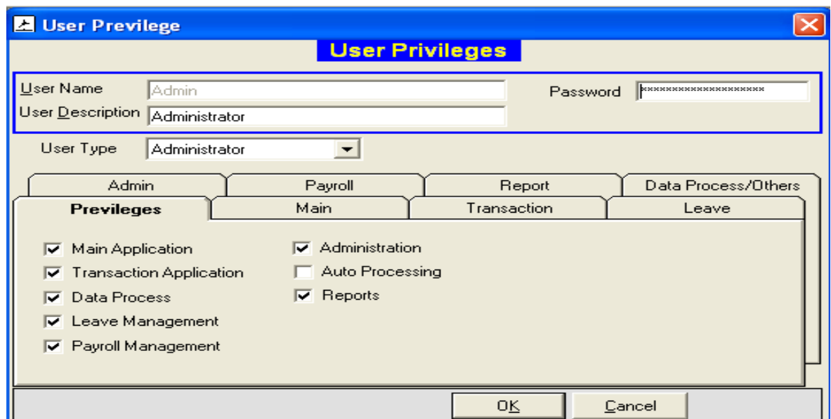
Figure 55: User Privilege
