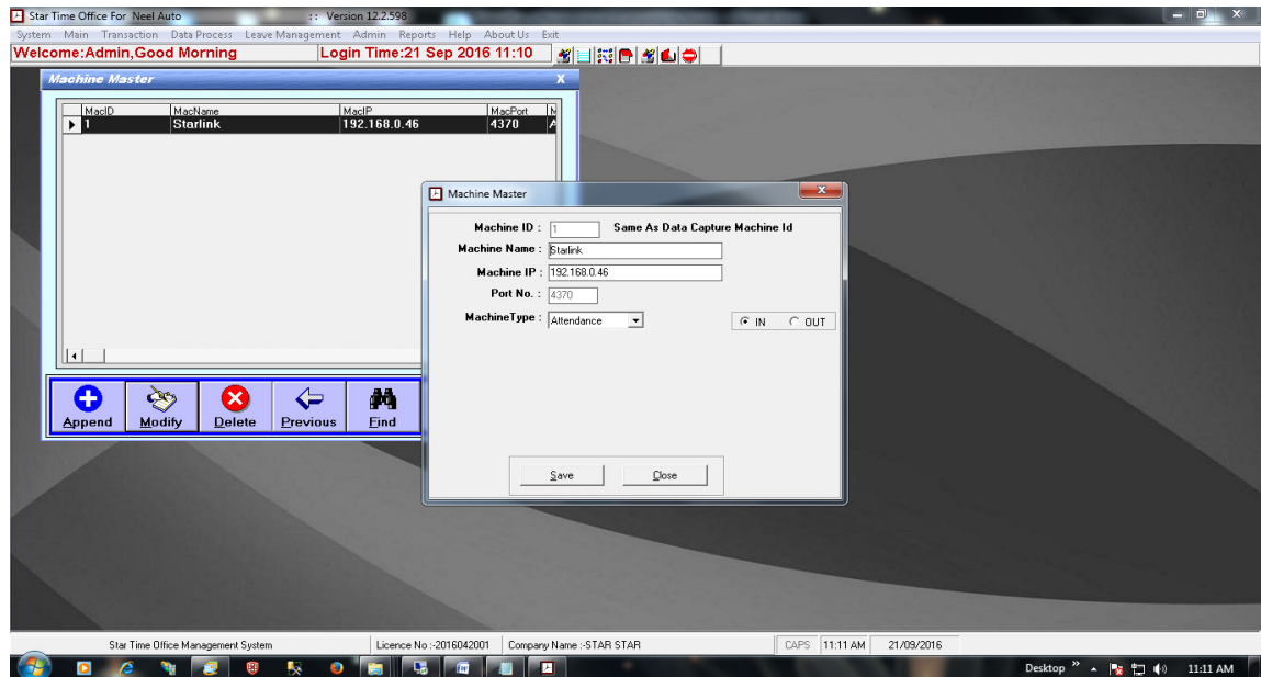
Figure 31: Machine Setting
