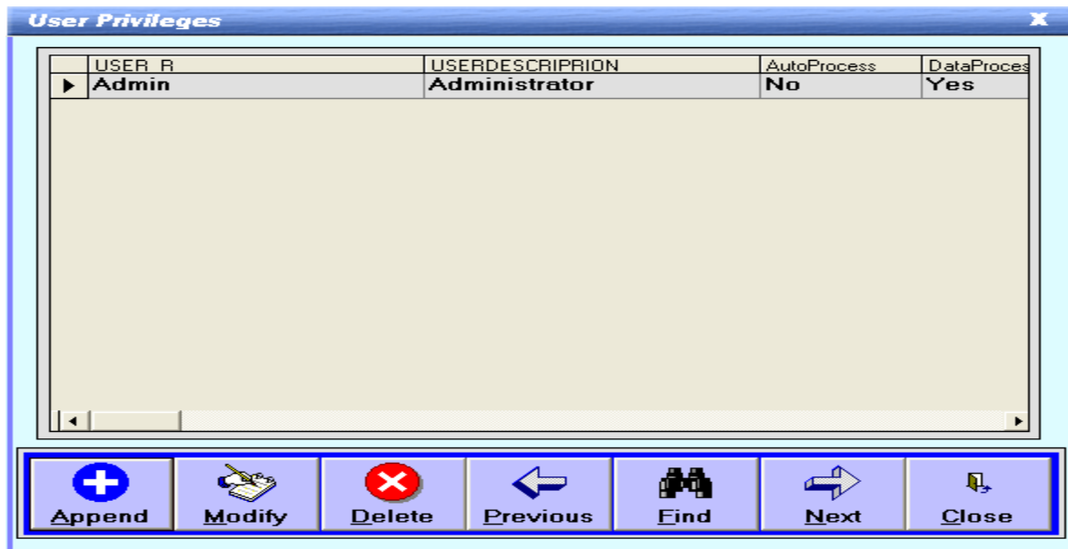
Figure 54: User Privilege-1
