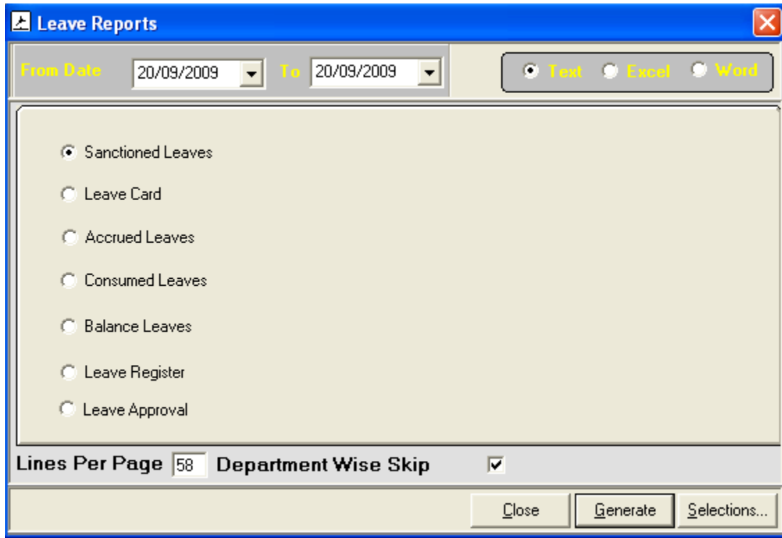
Figure 62: Leave Reports
