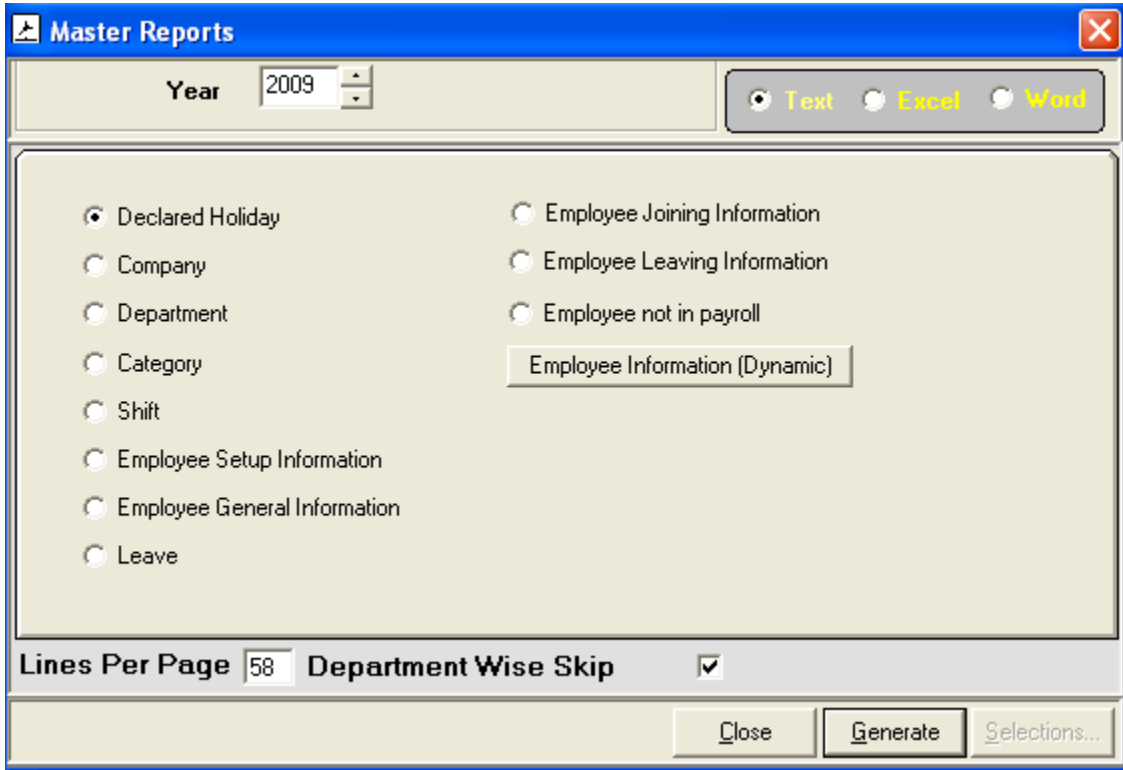
Figure 63: Master Reports
