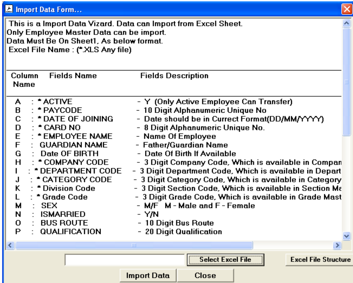
Figure 7: Import Data
