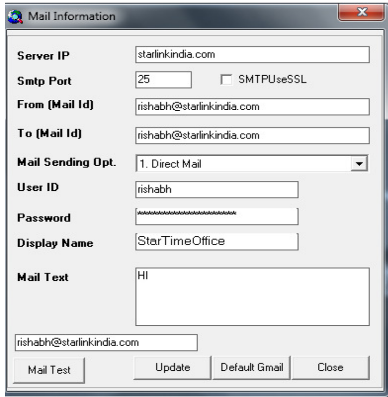
Figure 58: Mail Setting
