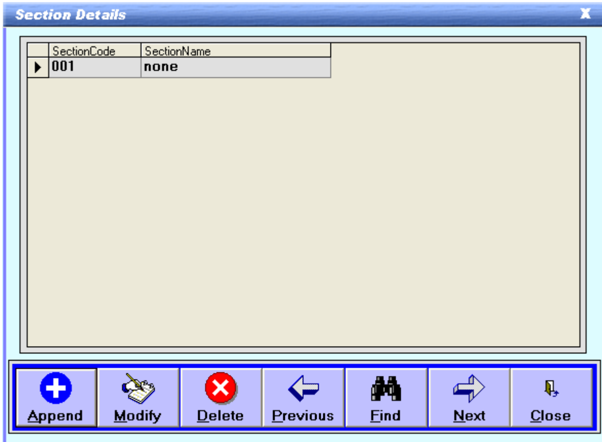
Figure 13: Section Master-1
