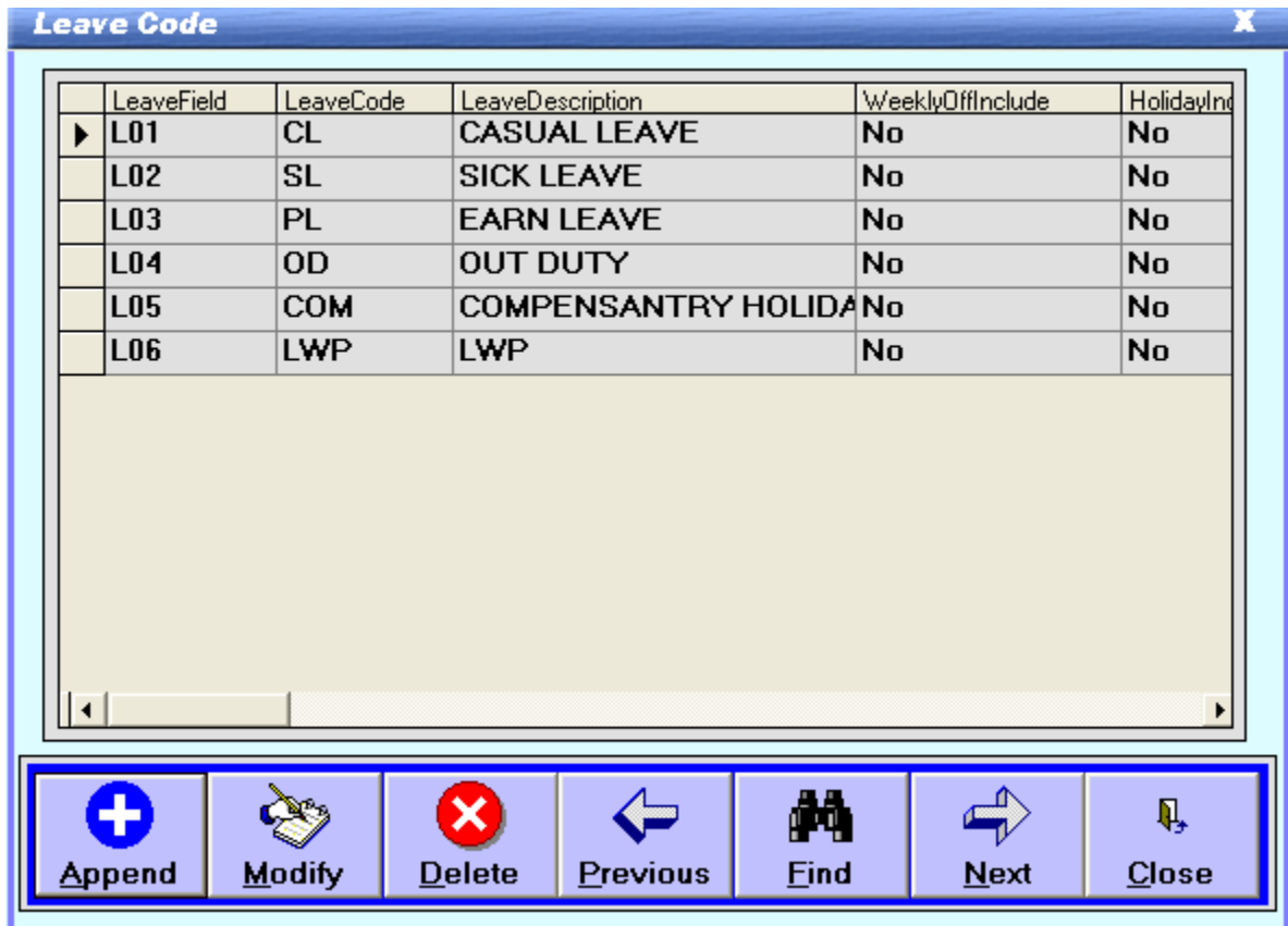
Figure 46: Leave Master
