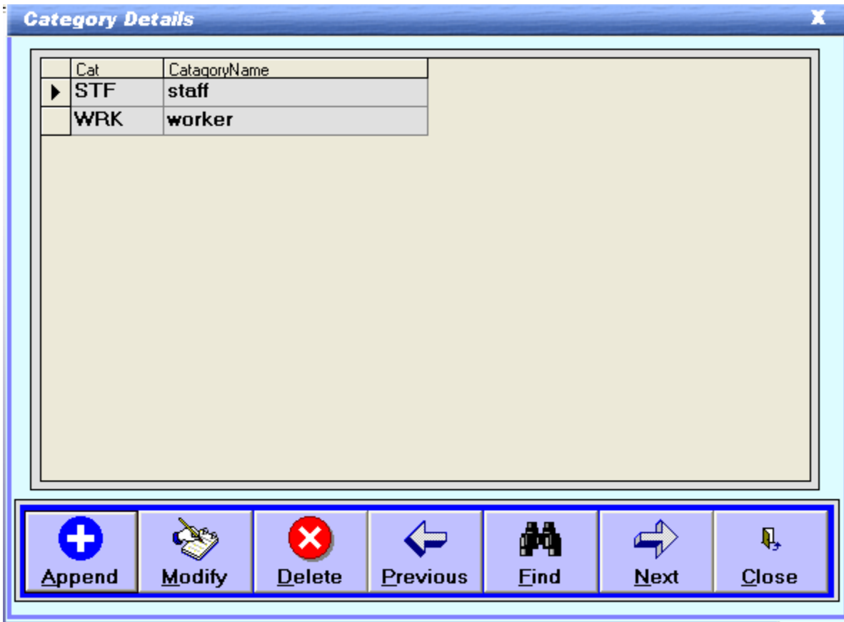
Figure 17: Category Master -1
